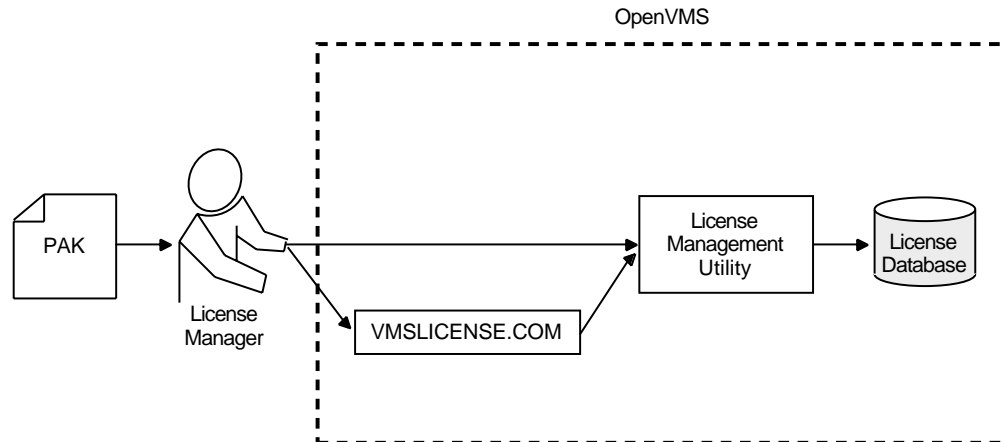
Figure 2–2 From a PAK to the License Database
