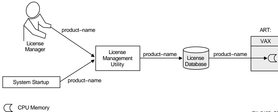
Figure 2–4 Loading a License
