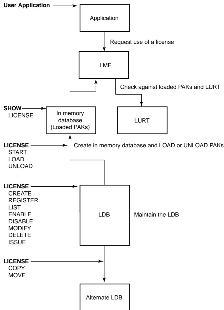
Figure 1–1 The Licensing Model
